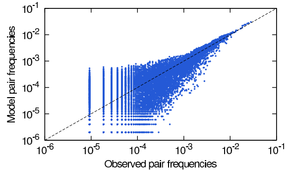
Figure 2. Model VS observed pair frequencies. The observed ones are from the corpus (WeimarJazzDatabase). The model frequencies come from a K_{max} = 10 model.
