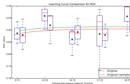
Figure 4. Area under the ROC curve predictive performance of a SGD SVM as a function of the fraction of ribozyme sequences.
