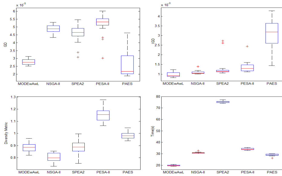
Figure 6: Performance comparisons of five algorithms in term of GD, IGD and \Delta metrics for DAX 100 dataset.
