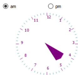
Figure 3: The user can select an hour on the clock interface to start the smooth zooming and panning animation to the new hour. Selecting the ‘pm’ radio button changes the clock to the afternoon hours.
