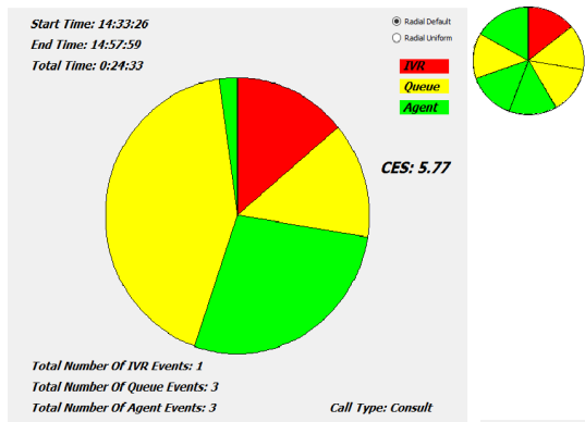
Figure 7: This shows the radial method for breaking down the call events of a single call. Starting at the midnight position and moving clockwise, the red segment shows the proportion of time spent in the IVR. Yellow events show queue time and green events shows agent time. The right radial plot shows the uniform view whereby each event is drawn as the same size to reveal any zero second events.
