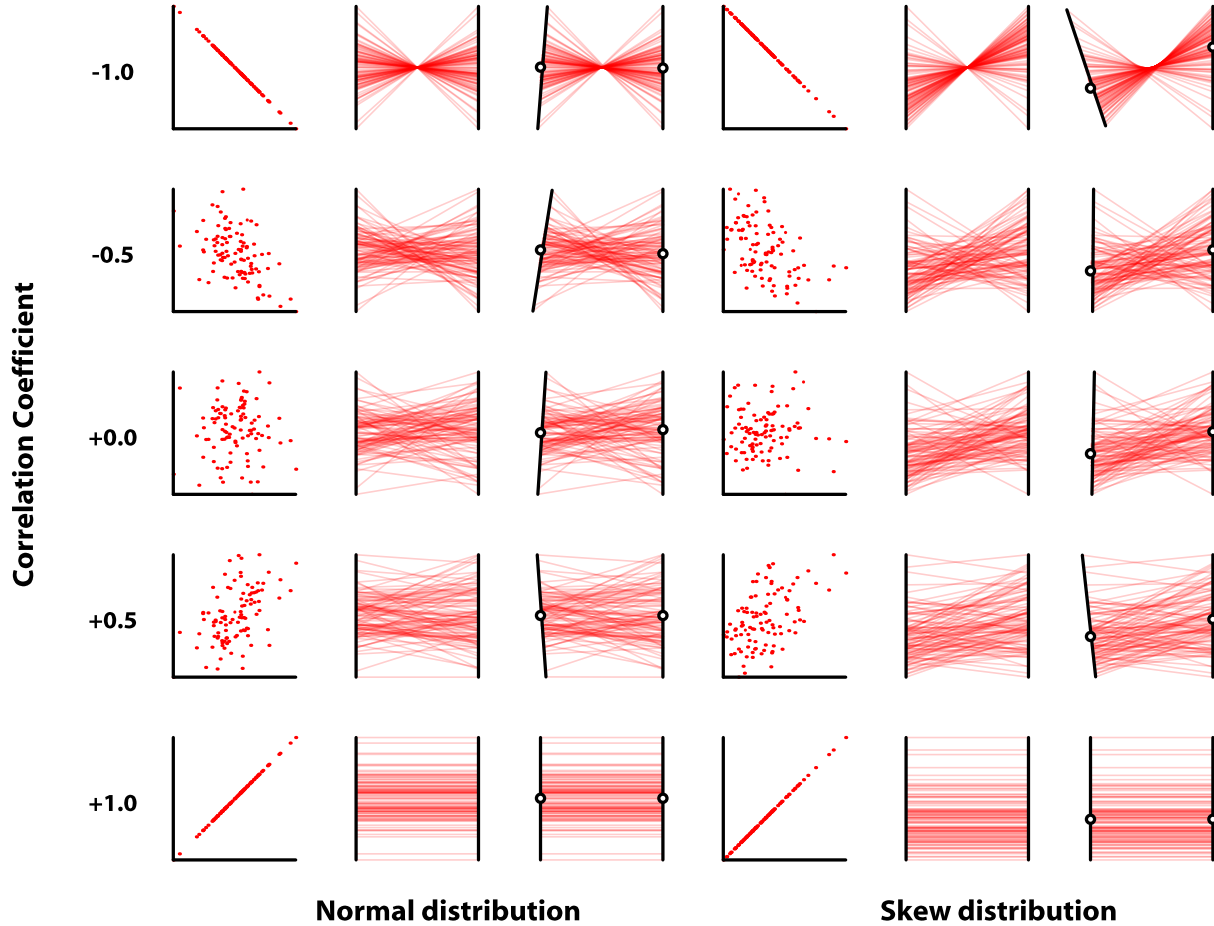
Figure 2: Comparisons between scatterplots, PCPs and force-directed PCPs for two dimensions using synthetic data generated with known skew and correlation. The first three columns show data with the given correlation where both variables follow a normal distribution, while the last three columns show data for which one axis has a skew-normal distribution and the other is normally distributed. In neither case is there a large movement of the axes, due to our choice of pivot position, and this places the focus for exploration on user interaction.
