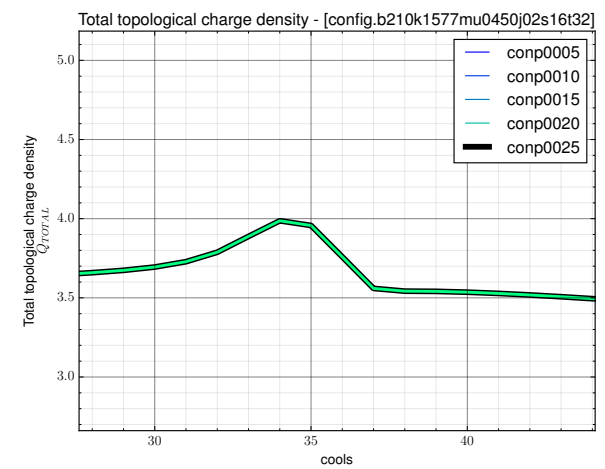
Figure A.13: Physicists look for a flattening of the topological charge density indicating stability. A short lived peak in the graph can characterise an instanton falling through the lattice or an instanton-anti-instanton annihilation.
