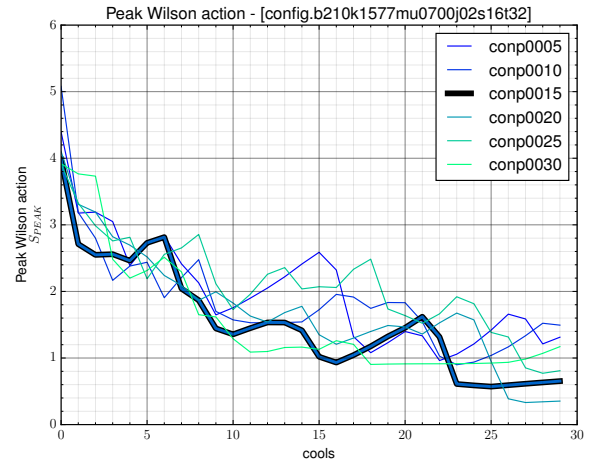
Figure A.9: Spikes in the action graph indicate the spreading and smoothing of an instanton, followed by a merging of two or more distinct objects.
