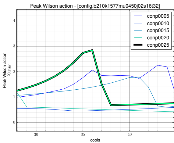
Figure A.12: An instanton falling through the lattice is characterised by the relatively high gradient drop in the peak action graph, this can be cross referenced with the topological charge density graph.
