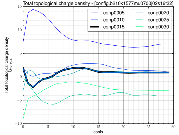
Figure A.8: A flattening in the topological charge density indicates a region of stability that can be cross referenced against the peak action graph to select interesting levels of cooling for study.
