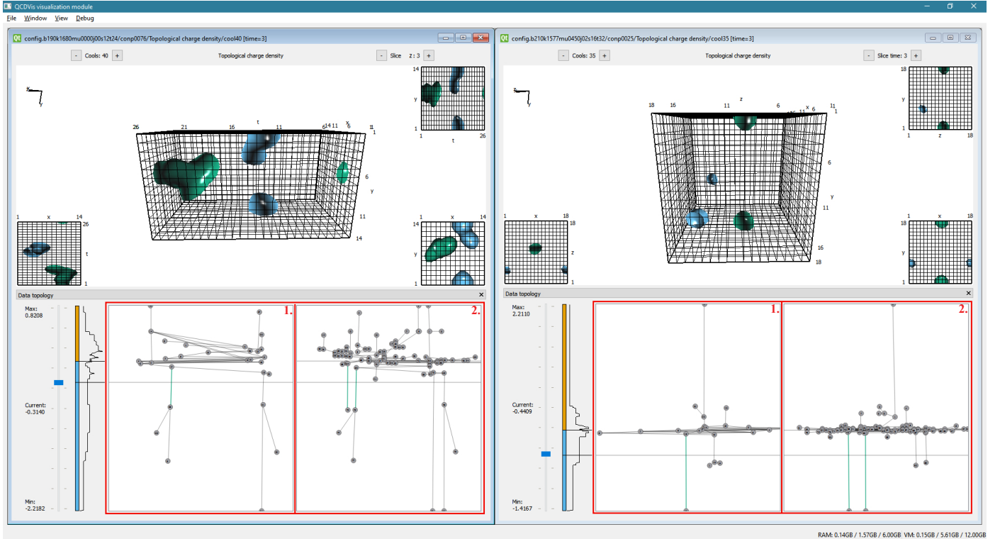
Figure 4: Left: An object (green) crossing a periodic boundary on the t axis, a second object (blue) crosses on the y boundary. Right: Two objects crossing the x and y axes in a time-slice of topological charge density. Both visualisations are shown alongside their Reeb graph (1.) and the contour Tree (2.) representations to illustrate the difference in these topological structures when dealing with periodic boundaries.
