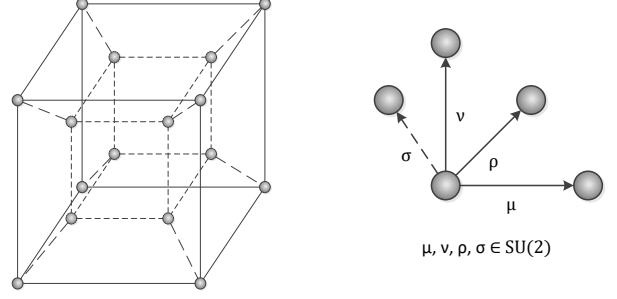
Figure A.6: Placement of data on the 4D lattice edges ( \sigma is a link in t dimension).
