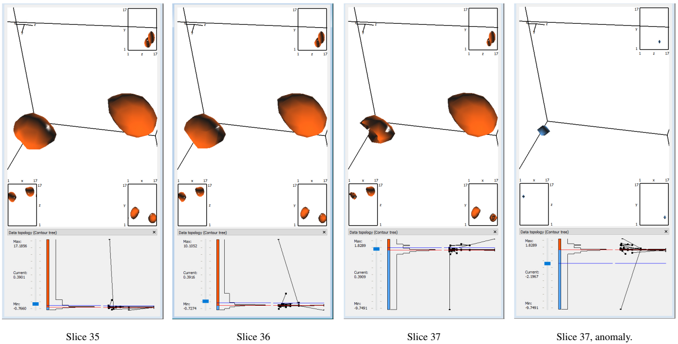
Figure A.11: Cooling slices 35, 36 and 37, shown at the same isovalue. At cooling step 37 the large object on the left starts to deform and disappears, being replaced by a global minima (right image). This phenomena can also be observed in the contour trees for each cooling phase.
