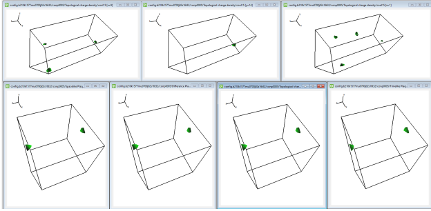
Figure A.10: Top: user examining the position of Topological Charge Density minima (anti-instanton) in the xyt , xzt and yzt sub-volumes. Bottom: comparing the location of peak Wilson action and Topological Change Density minima in xyt sub-volumes.
