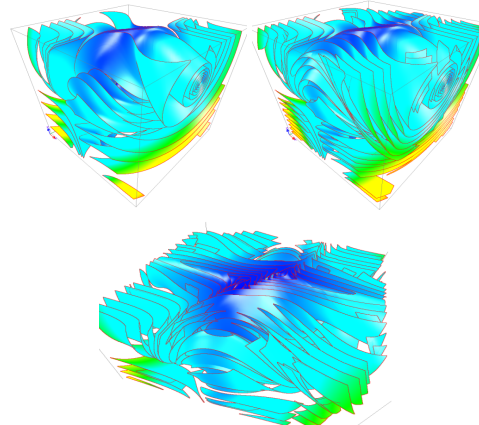
Figure 10: This visualization of the Lorenz attractor shows the effect of denser seeding. The top left image shows boundary seeding at 5 intervals. The top right image shows interior seeding using d_{sep} = 5.0 . The bottom image is clipped revealing the inner flow characteristics.
