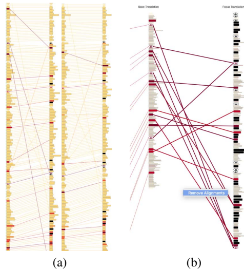
Fig. 2. (a) On the left, the alignments without applying the confidence value threshold. On the right, the effect of applying a threshold ( \kappa = 0.75 ). Some of the diagonal edges are removed. (b) A screenshot of the deletion action when the user selects multiple alignment edges.
