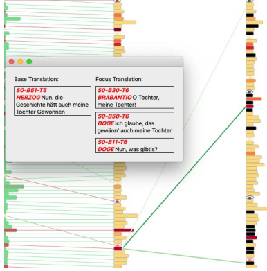
Fig. 3. A screenshot of the top three candidate segments for a user-chosen T_B segment (RE). The candidate segment edges are rendered in green and the saturation of the color represents the rank of the candidate segments. The order of the segments is based on the ranking of the each segment.
