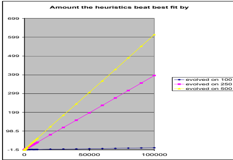
Fig. 1. The horizontal axis shows the number of pieces packed. The vertical axis shows the number of bins a heuristic beats best fit by. This is done for heuristics evolved on problem instances of three different sizes (containing 100, 250 or 500 pieces). This horizontal scale goes up to 100000 pieces, much larger than the number of pieces contained in the problem instances used in the training phase. These results are averaged over 30 heuristics over 20 problem instances.
