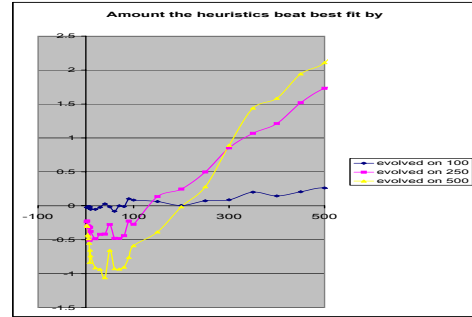
Fig. 2. The horizontal axis shows the number of pieces packed. The vertical axis shows the number of bins a heuristic beats best fit by. This is done for heuristics evolved on problem instances of three different sizes (containing 100, 250 or 500 pieces). Note that the horizontal scale covers the size of the training problem instances.
