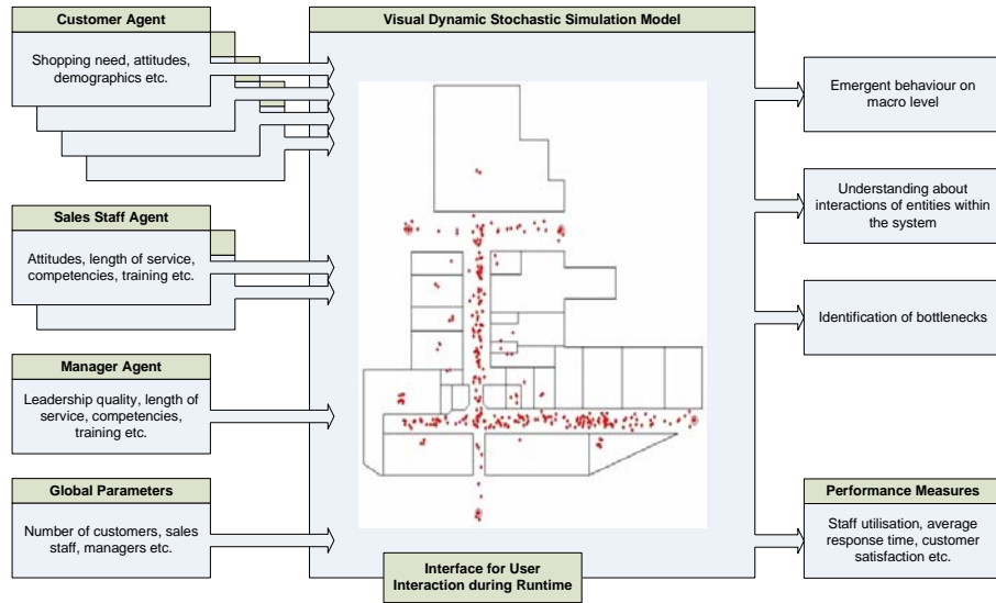
Figure 1. Conceptual model for the simulator
