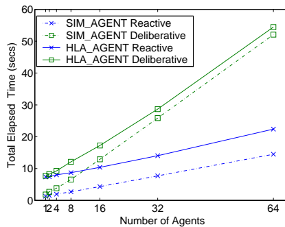
(a) Total elapsed times for 1-64 Reactive and Deliberative agents in SIM_AGENT and HLA_AGENT (single federate).
