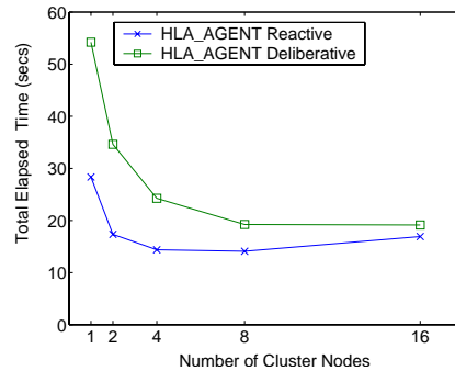
(b) Total elapsed times for an Agent Federate (64 Reactive and Deliberative Agents distributed over 1-16 nodes).
