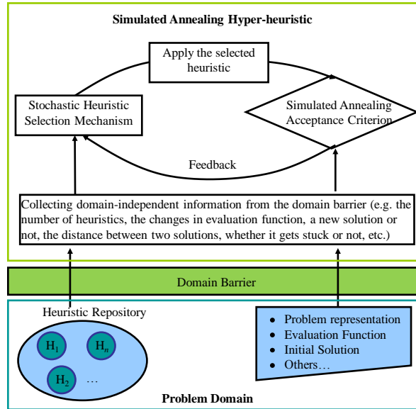
Fig. 3 Simulated annealing hyper-heuristic framework.
