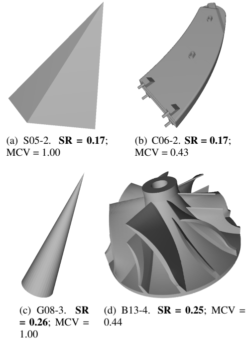
Figure 5. Comparison between parts with the same Spies Ratio but different MCV values.
