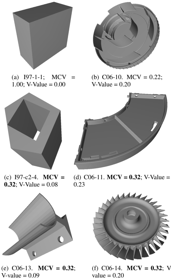
Figure 3. Comparison between a part with high MCV and low v-value to another with low MCV and comparatively high v-value; and comparisons between parts sharing the same values of MCV but different v-values.
