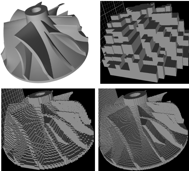
Figure 1. An example from the Baumers et al. [9] rasterized in resolutions of 20, 100 and 200 voxels.
