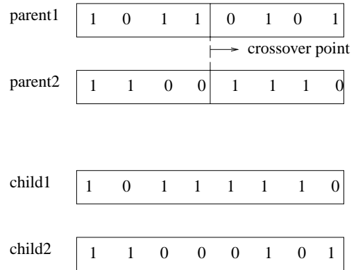
Figure 20. Crossover operation.
