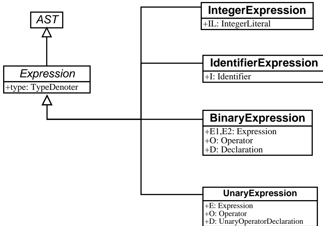
Figure 2: Expression ASTs
