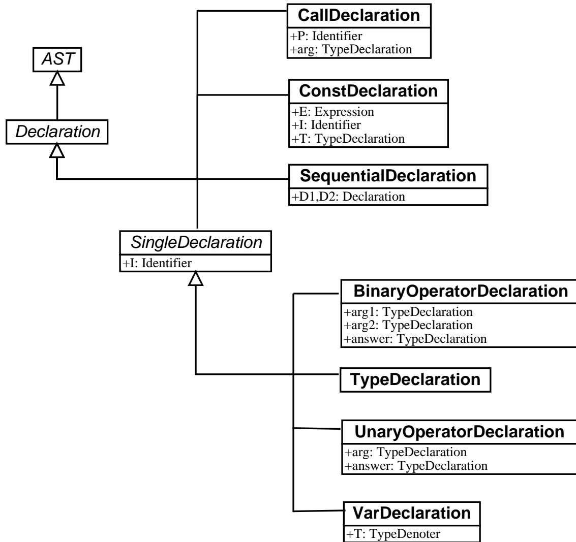
Figure 3: Declaration ASTs
