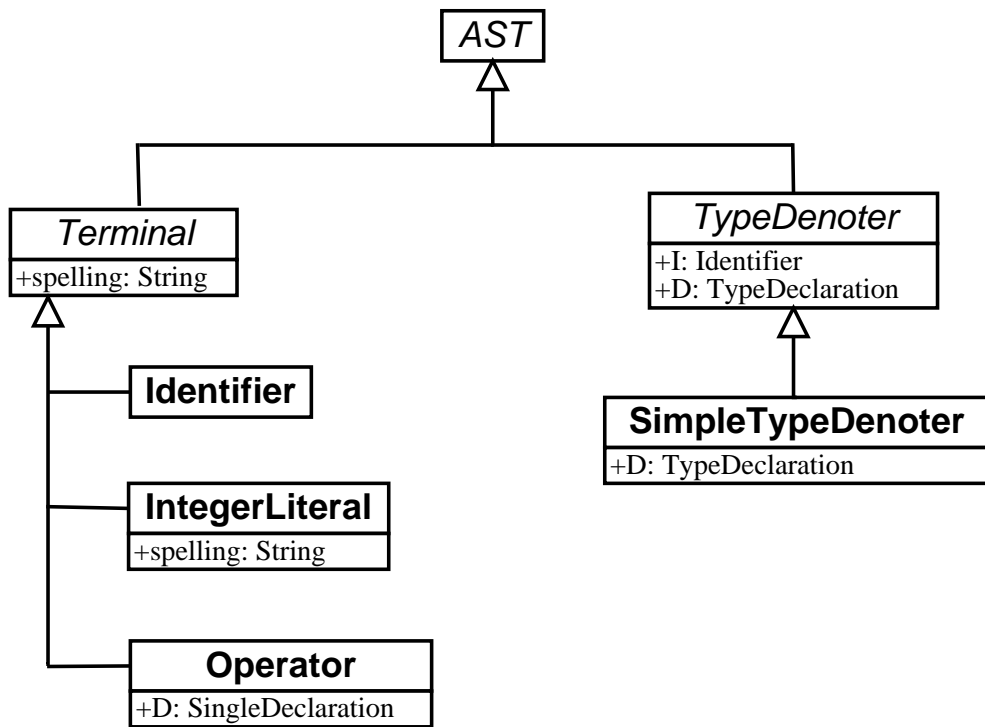
Figure 4: Terminal and TypeDenoter ASTs
