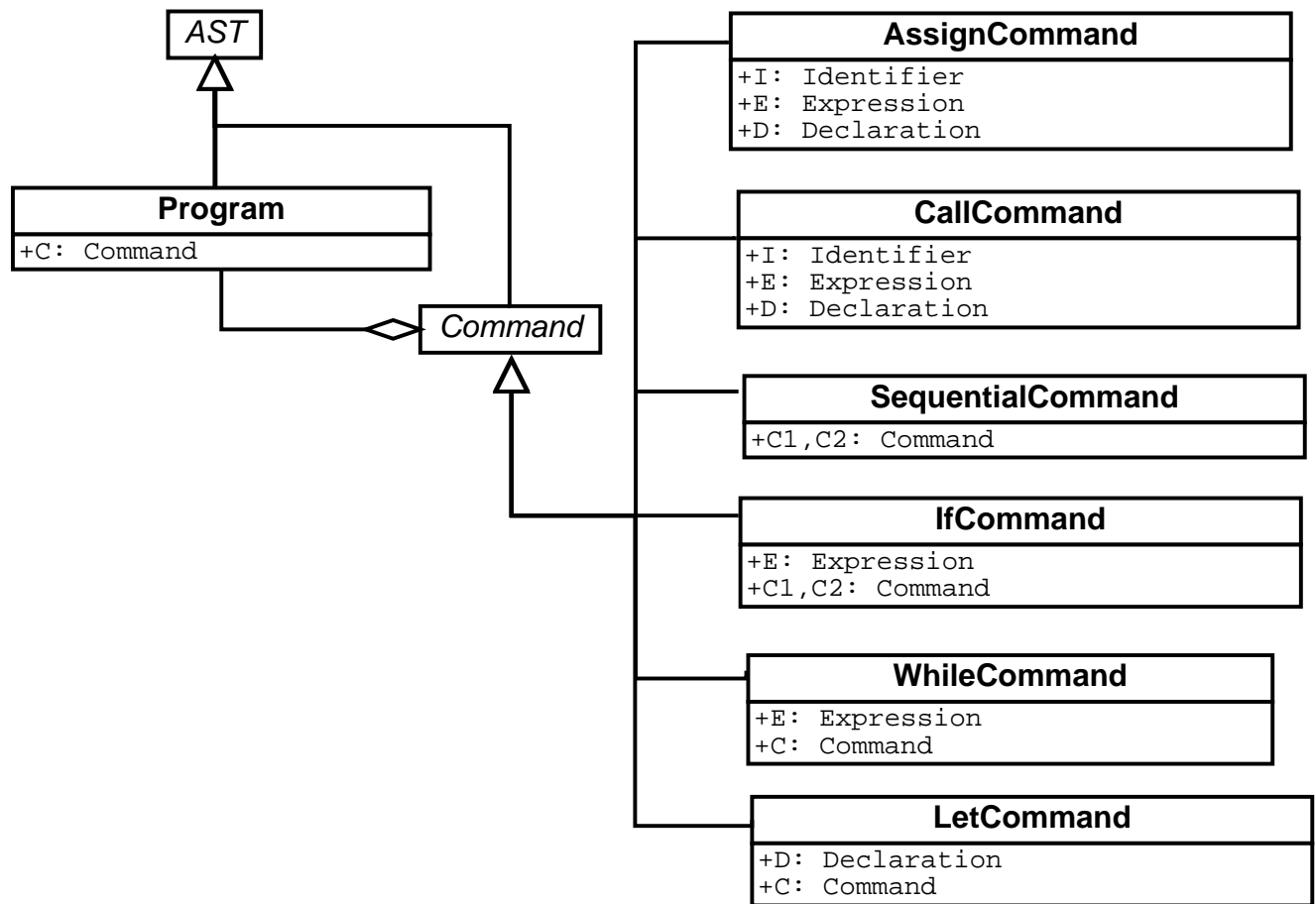
Figure 1: Program and Command ASTs
