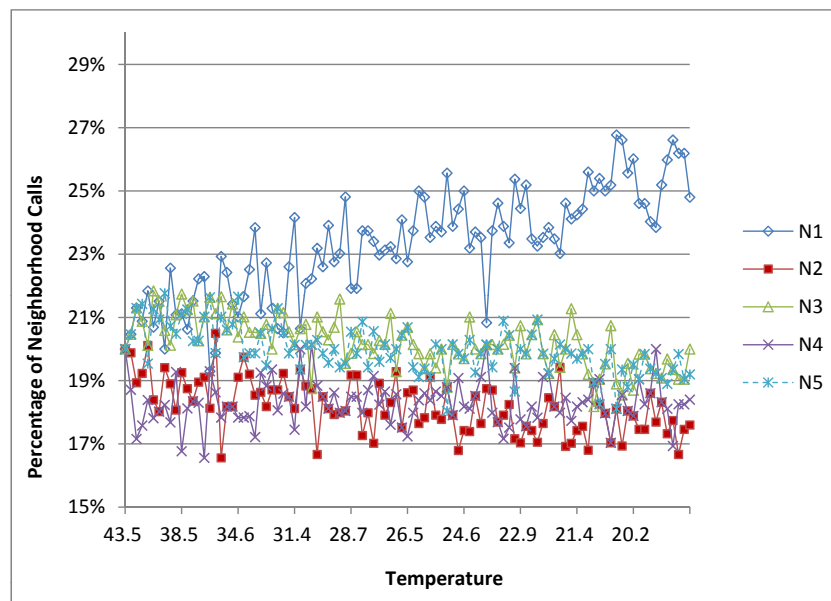
Fig. 8. Adaptation of neighbour calls at different annealing temperatures (For instance n50m5_01. Distributions for other instances are similar.)
