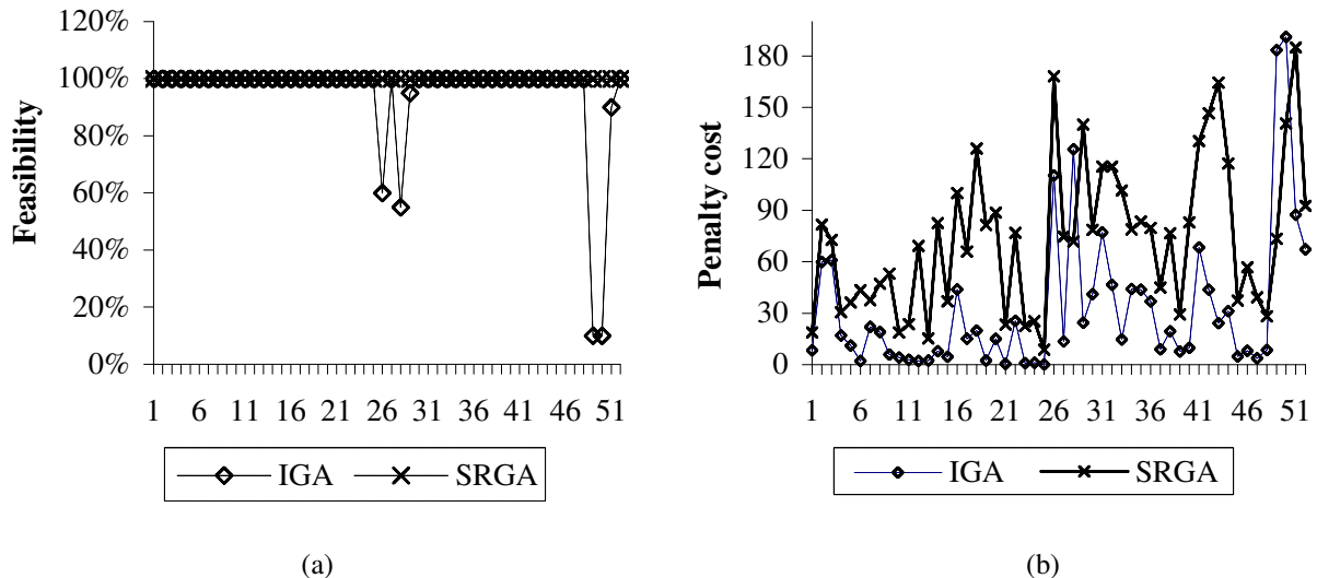
Fig. 2. A comparison of stochastic ranking genetic algorithm (SRGA) with indirect genetic algorithm (IGA) by [1]: (a) Percentages of feasible solutions obtained among 20 runs. (b) Average objective value over 20 runs.
