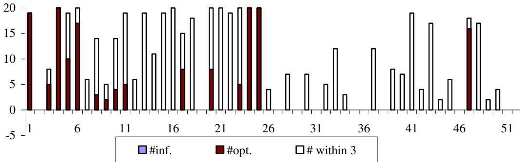
Fig. 6. Detail results by EDA with "ant-miner" heuristics
