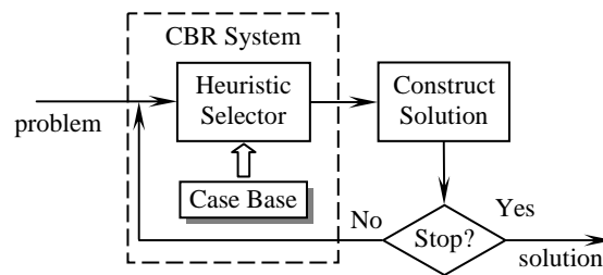
Figure 3 The case based heuristic selection approach
